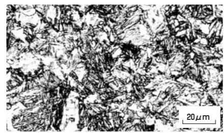
(c) ドリルねじ (0.19% C鋼, HV: 388)
